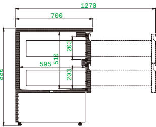
S901 S/S Top 2 × GN1/2 S901 S/S Top 4 × GN1/2
