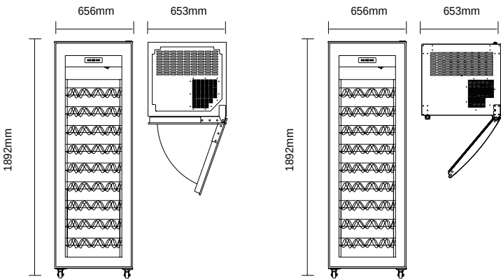
Front flat glass door M-400L-2
