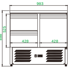
S901 S/S Top 2 × GN1/2
