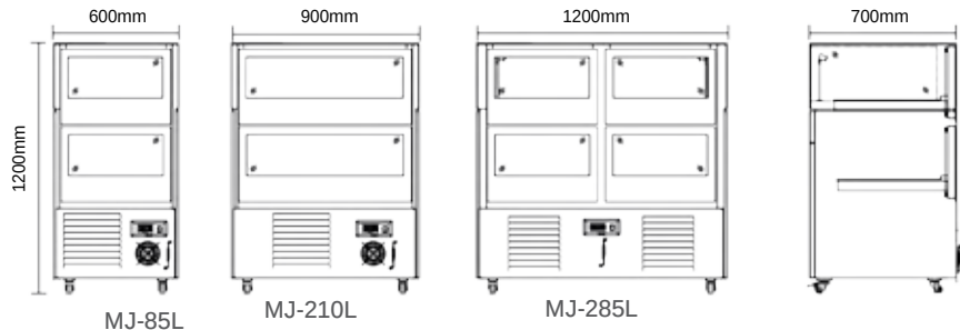
Glass drawers (The drawer's laminate is provided with luminous lighting.)
